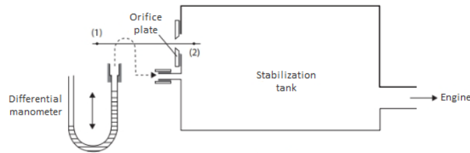
Figure 5. Schematic layout for measuring air consumption for the engine (Brunetti, 2018).
