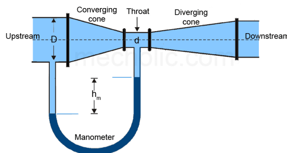
Figure 3. Venturi tube (Mecholic, 2020)
