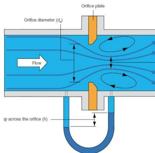
Figure 2. Orifice plate (Mohamed et al. , 2017)
